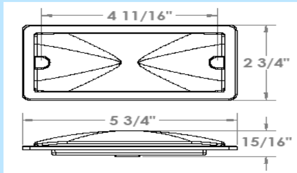
Mechanical Design
